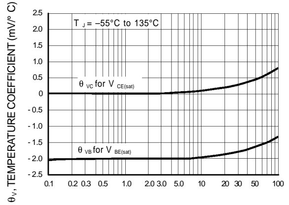
I_c , COLLECTOR CURRENT (mA) Figure 5. Temperature Coefficients
