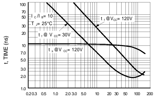
I_c , COLLECTOR CURRENT (mA) Figure 9. Turn-Off Time
